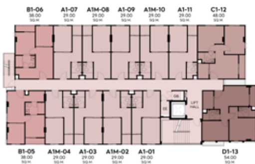
4 th - 6 th FLOOR
