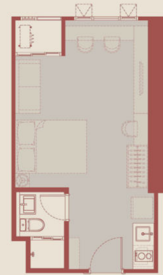
TYPE B1M 26.50 SQ.M.
