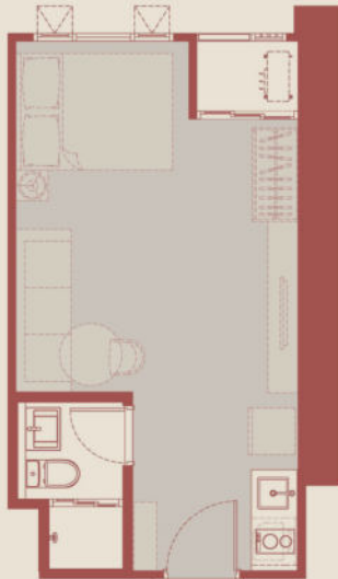
TYPE A2 24.00 SQ.M.
